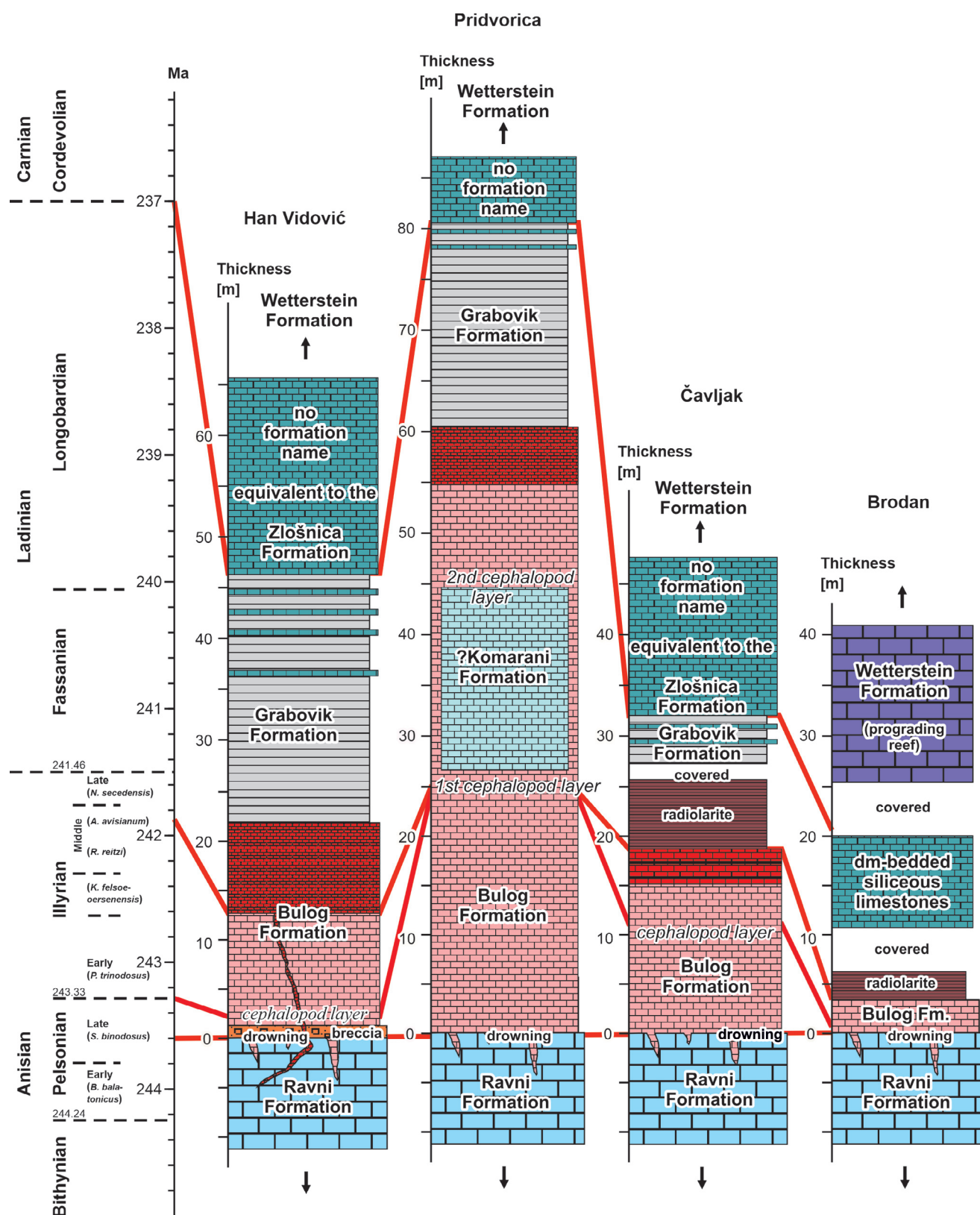
Fig. 23. Thickness and age correlation of the type-section Han Vidović and the sections Pridvorica, Čavljak, and Brodan (simplified columns). Absolute ages (Ma) from OGG et al. (2020). Sections Han Vidović and Pridvorica after SUDAR et al. (2023c), in cases corrected and modified on base of new data.
