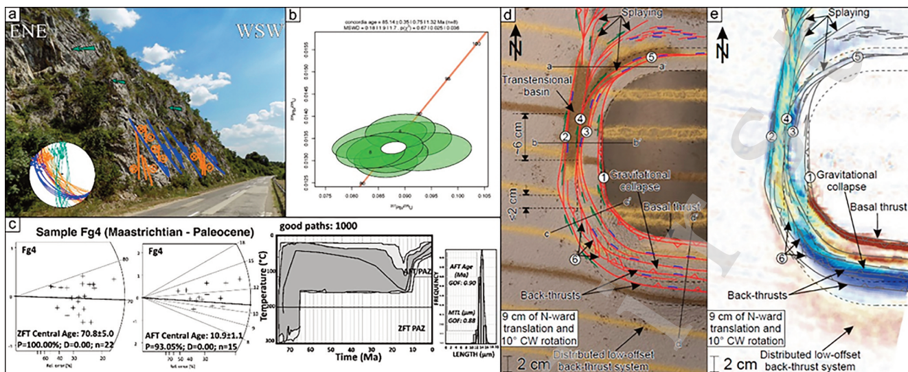
Fig. 4. Multi-disciplinary approach: a) Field structural analysis (KRSTEKANIĆ et al., 2022); b) U/Pb absolute dating (BANJEŠEVIĆ et al., 2019, VELOJIĆ et al., 2020, 2023); c) Provenance study using detrital thermochronology (STOJADINOVIĆ et al., 2017); d, e) Analogue modelling of complex fault systems (KRSTEKANIĆ et al., 2021).
