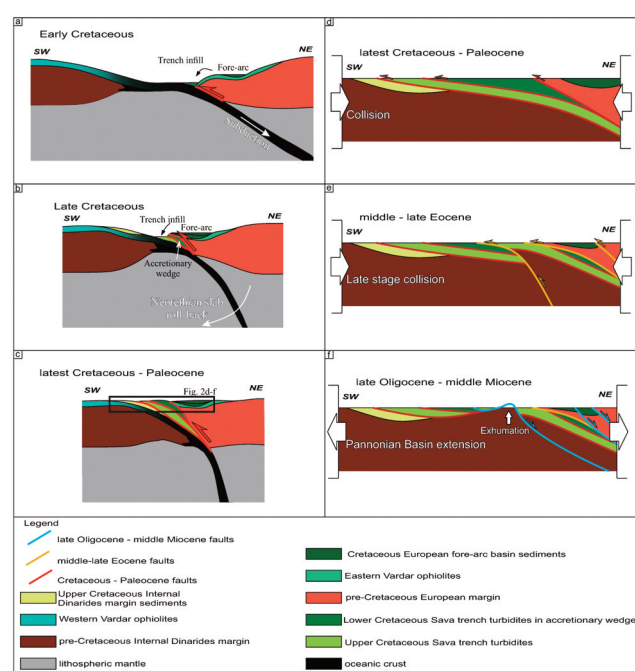
Fig. 2. Conceptual sketch (not to scale) of the Adria-Europe convergence zone evolution in central Serbia during Cretaceous–Miocene times (modified after STOJADINOVIC et al., 2022): a) The Early Cretaceous E-ward subduction of the Adria lower plate beneath the overriding Europe-derived units, within the Sava subduction system; b) The Late Cretaceous accelerated subsidence in the Sava subduction system due to the Neotethyan slab rollback; c, d) Latest Cretaceous to Paleocene continental collision and WSW-ward thrusting of the European fore-arc basin and Lower Cretaceous Sava trench sediments over the Upper Cretaceous Sava trench turbidites and Internal Dinarides margin deposits; e) Middle to late Eocene out-of-sequence thrusting and exhumation of the Upper Cretaceous Sava trench turbidites underneath the overlying Lower Cretaceous Sava trench sediments; f) Oligocene–Miocene extensional reactivation of segments of the inherited thrusts and exhumation of the Adria lower plate.
